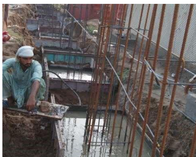
246-Foundations of Boundary Wall
